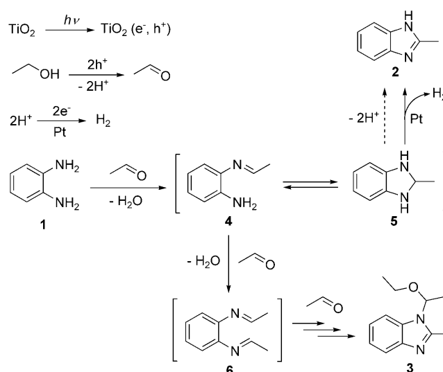
Scheme 2. Proposed mechanism for the one-pot synthesis of benzimidazole promoted by a Pt@TiO 2 catalyst under photoirradiation.
