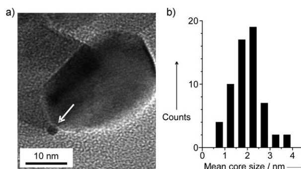
Figure 1. a) TEM micrograph of Pt(0.2)@TiO 2 and b) size distribution of platinum particles on Pt(0.2)@TiO 2 .
